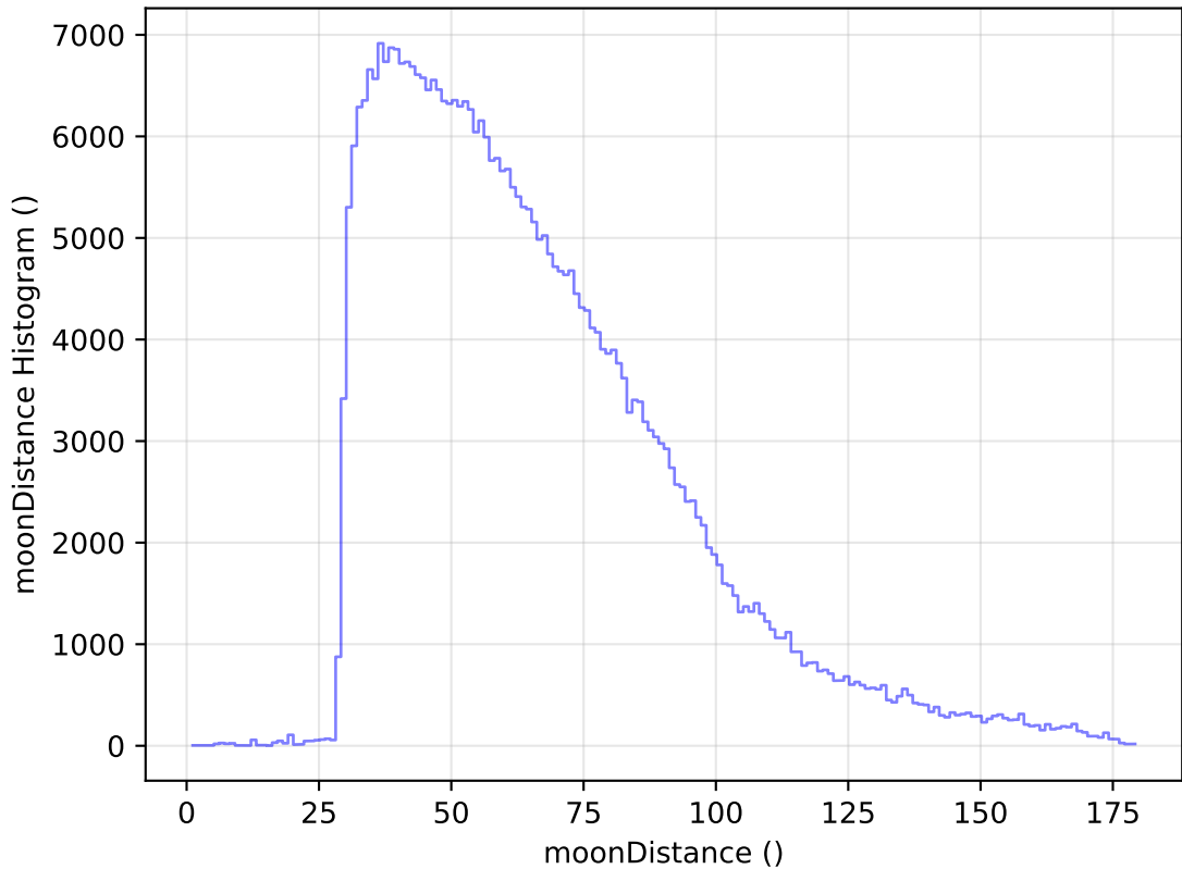
too_elab_r32_d2_ugrizy_v3.4_10yrs All sky y band: moonDistance Histogram
