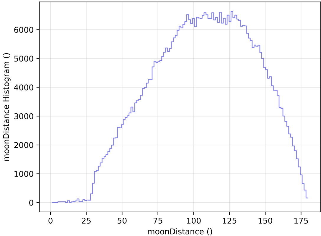
too_elab_r32_d2_ugrizy_v3.4_10yrs All sky r band: moonDistance Histogram
