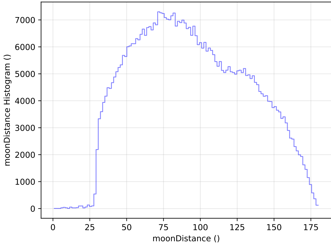
too_elab_r32_d2_ugrizy_v3.4_10yrs All sky i band: moonDistance Histogram
