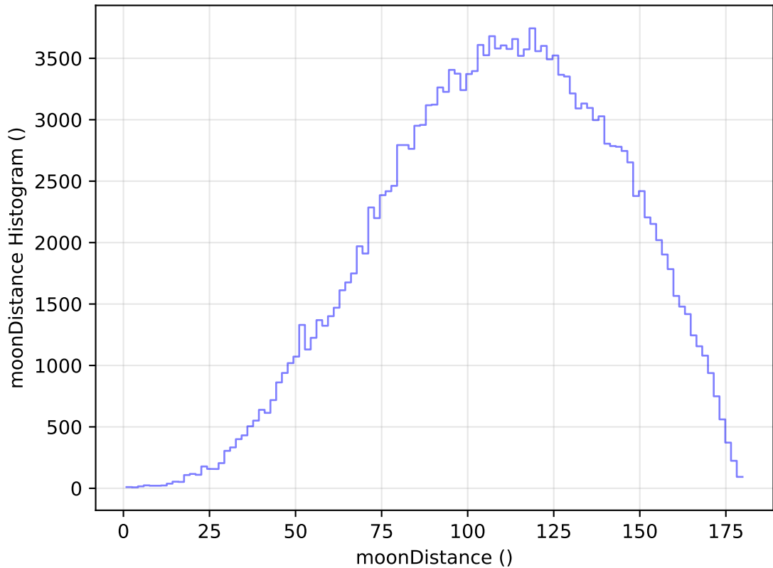
too_elab_r32_d2_ugrizy_v3.4_10yrs All sky g band: moonDistance Histogram
