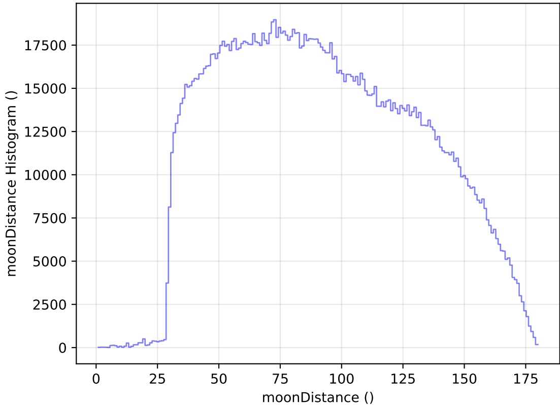
too_elab_r32_d2_ugrizy_v3.4_10yrs All sky all bands: moonDistance Histogram
