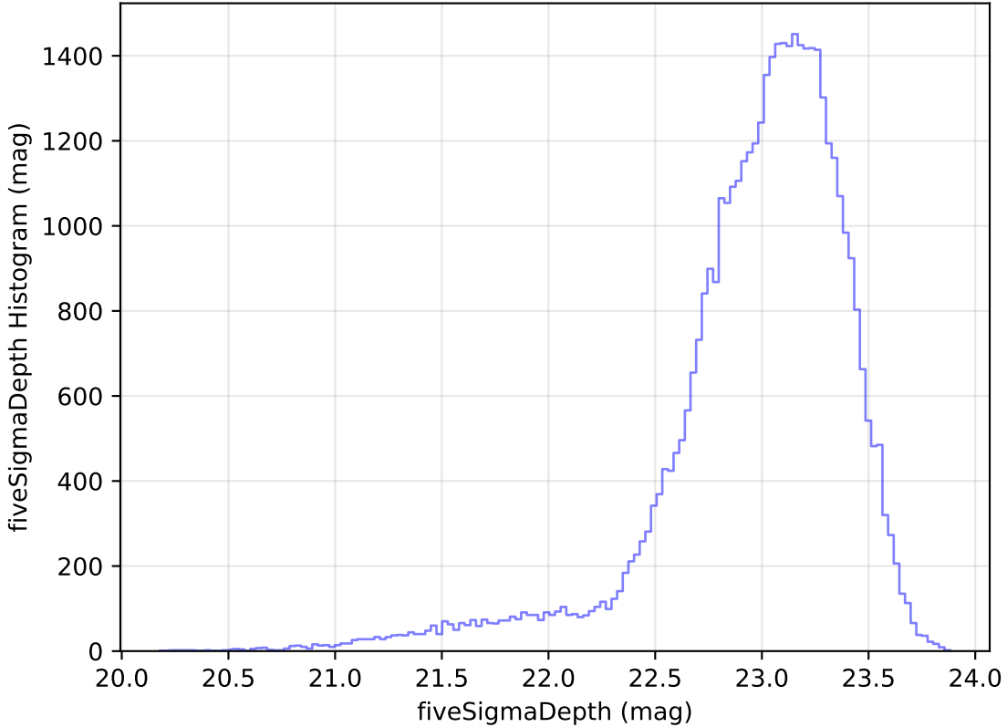
too_elab_r32_d2_ugrizy_v3.4_10yrs Yr 1 z band: fiveSigmaDepth Histogram
