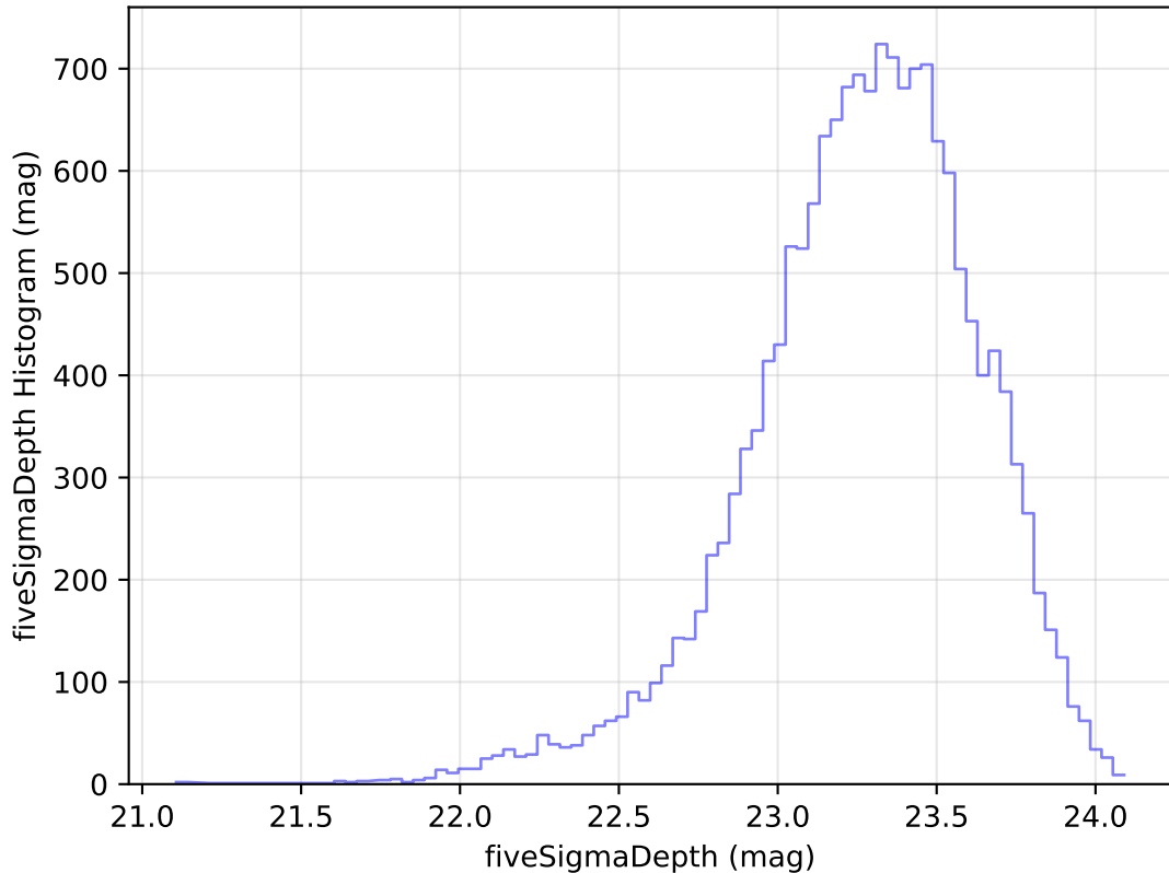
too_elab_r32_d2_ugrizy_v3.4_10yrs Yr 1 u band: fiveSigmaDepth Histogram
