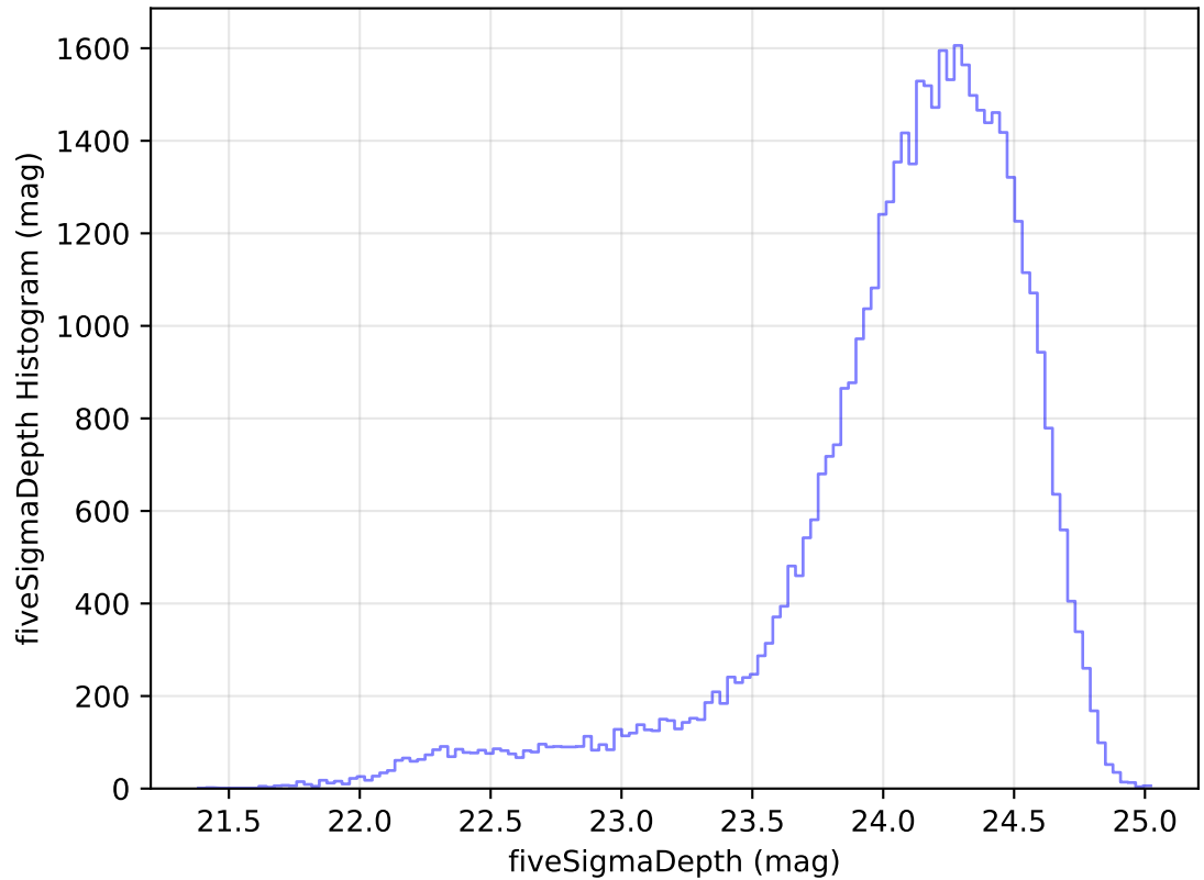
too_elab_r32_d2_ugrizy_v3.4_10yrs Yr 1 r band: fiveSigmaDepth Histogram
