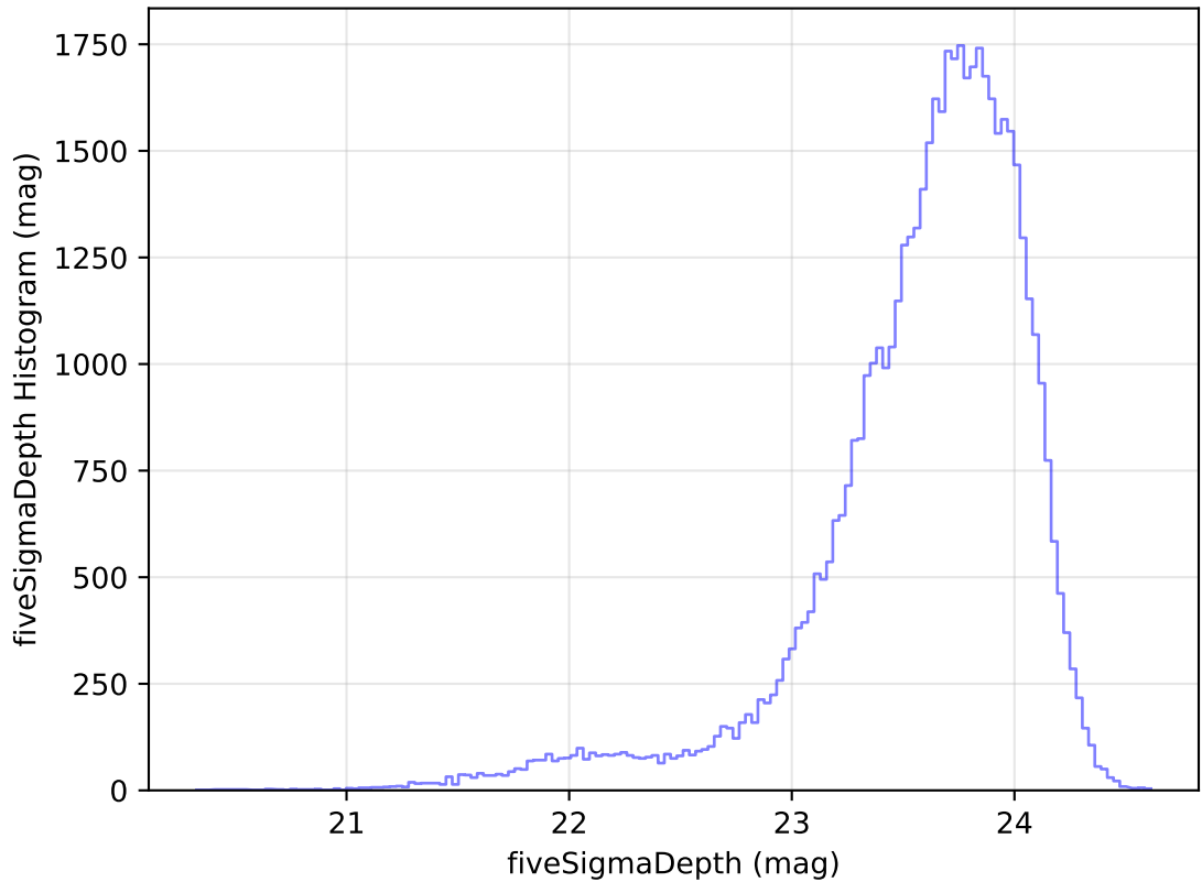
too_elab_r32_d2_ugrizy_v3.4_10yrs Yr 1 i band: fiveSigmaDepth Histogram
