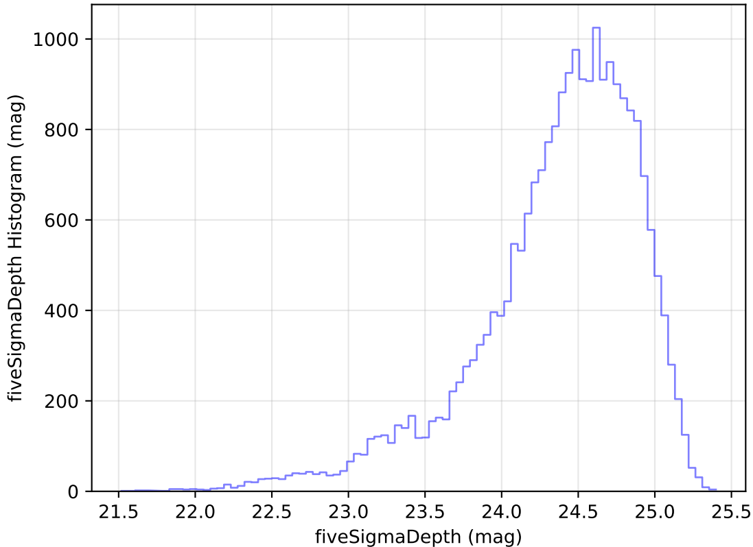
too_elab_r32_d2_ugrizy_v3.4_10yrs Yr 1 g band: fiveSigmaDepth Histogram
