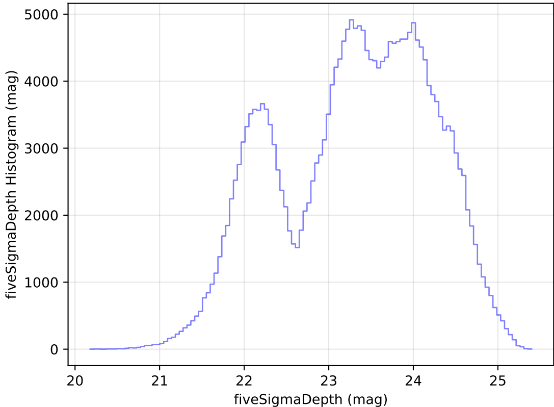
too_elab_r32_d2_ugrizy_v3.4_10yrs Yr 1 all bands: fiveSigmaDepth Histogram
