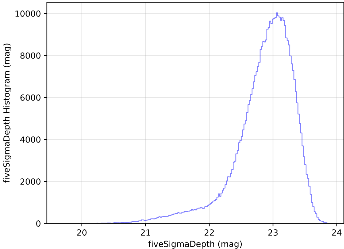
too_elab_r32_d2_ugrizy_v3.4_10yrs WFD z band: fiveSigmaDepth Histogram
