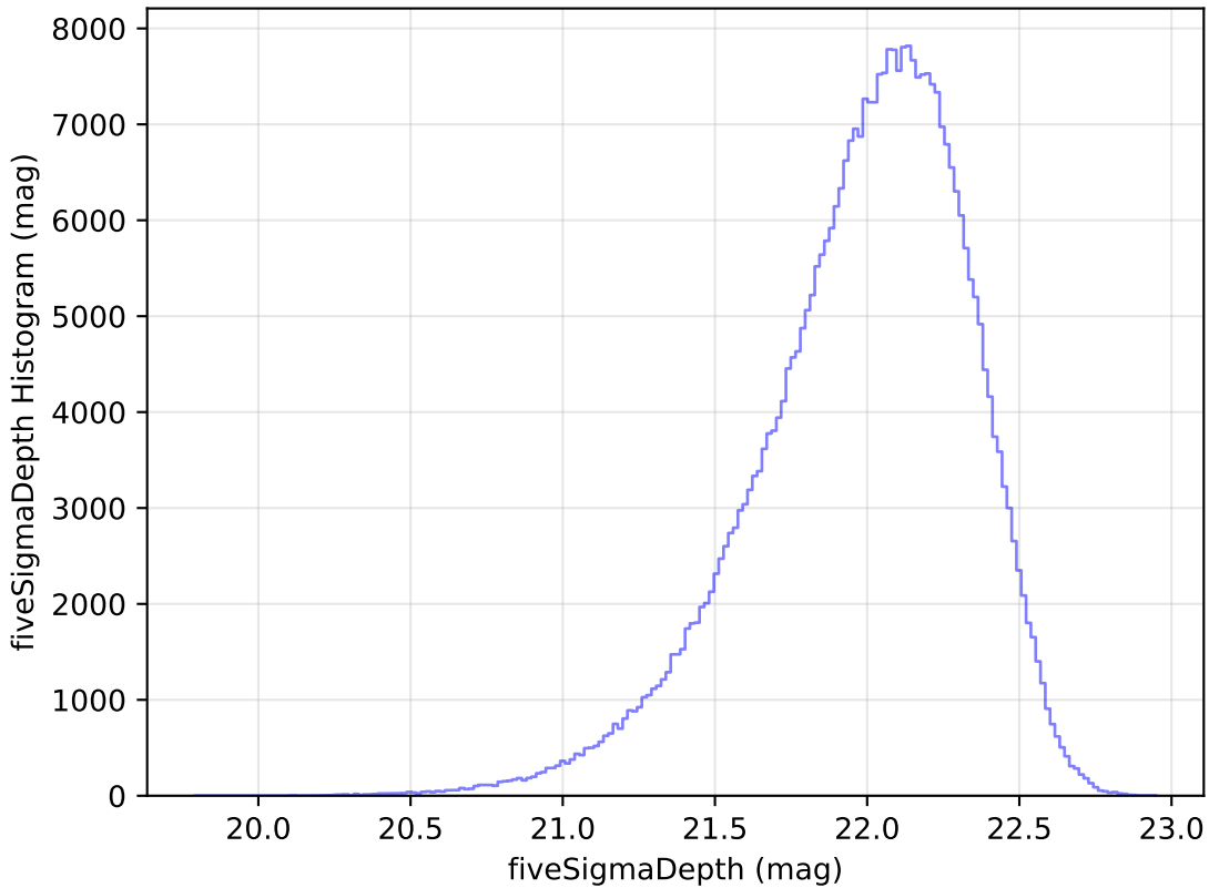
too_elab_r32_d2_ugrizy_v3.4_10yrs WFD y band: fiveSigmaDepth Histogram
