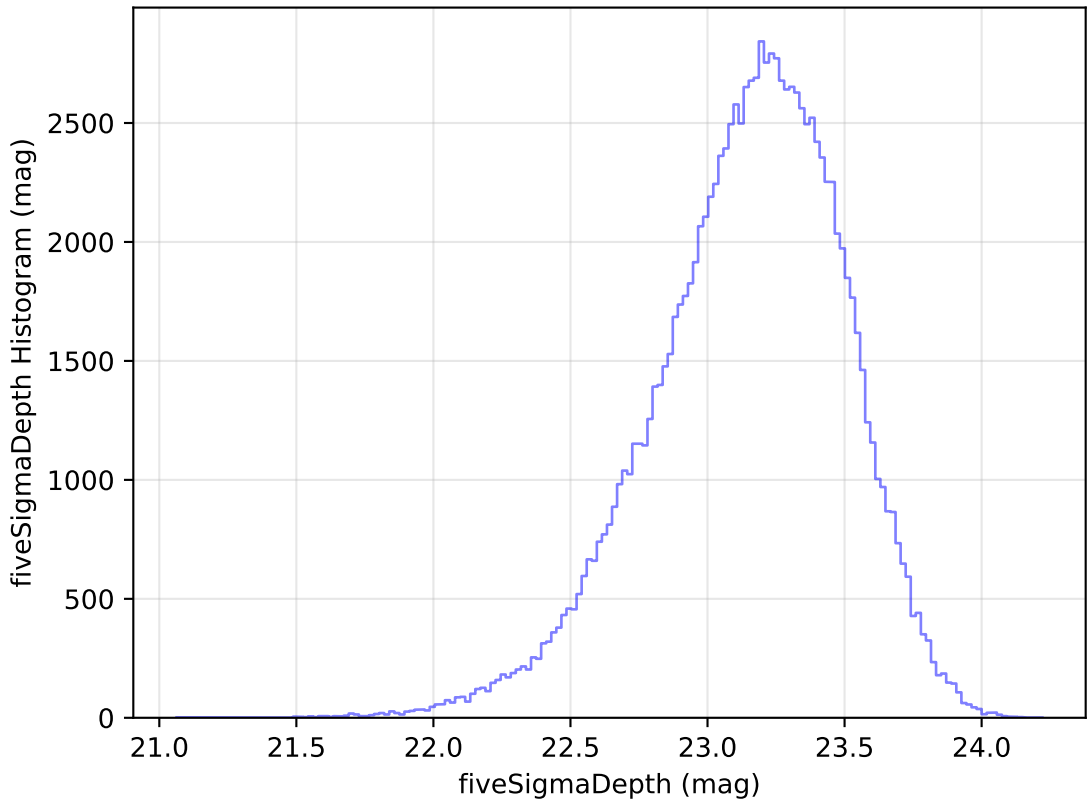
too_elab_r32_d2_ugrizy_v3.4_10yrs WFD u band: fiveSigmaDepth Histogram
