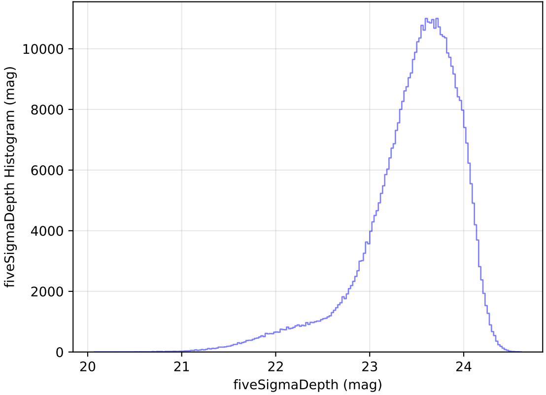
too_elab_r32_d2_ugrizy_v3.4_10yrs WFD i band: fiveSigmaDepth Histogram
