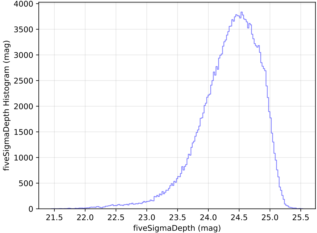
too_elab_r32_d2_ugrizy_v3.4_10yrs WFD g band: fiveSigmaDepth Histogram
