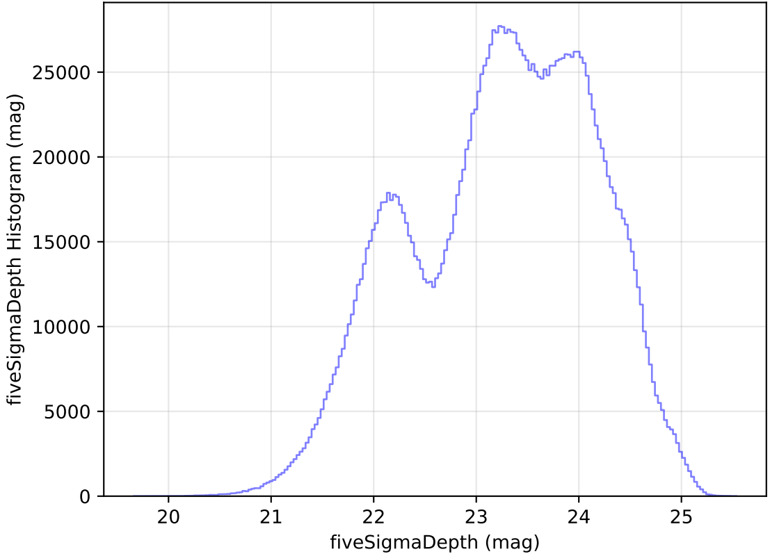
too_elab_r32_d2_ugrizy_v3.4_10yrs WFD all bands: fiveSigmaDepth Histogram
