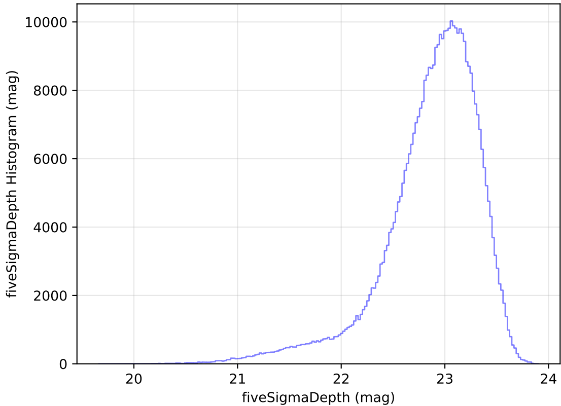
too_elab_r32_d2_ugrizy_v3.4_10yrs All sky z band: fiveSigmaDepth Histogram
