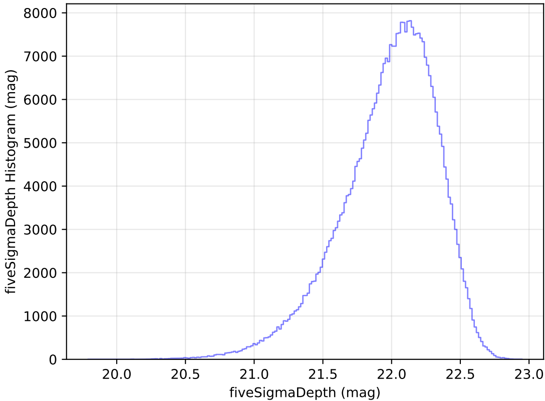
too_elab_r32_d2_ugrizy_v3.4_10yrs All sky y band: fiveSigmaDepth Histogram
