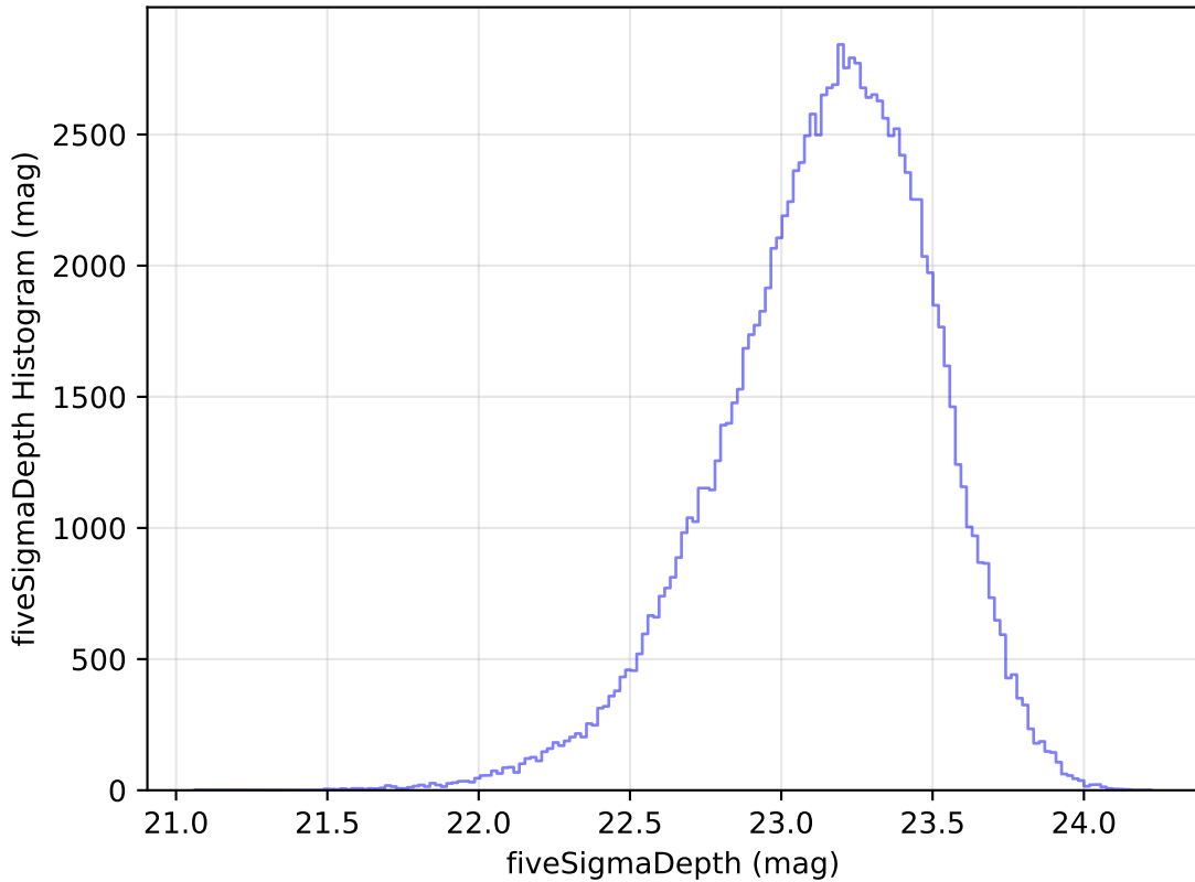
too_elab_r32_d2_ugrizy_v3.4_10yrs All sky u band: fiveSigmaDepth Histogram
