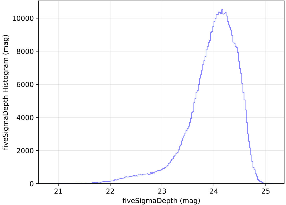
too_elab_r32_d2_ugrizy_v3.4_10yrs All sky r band: fiveSigmaDepth Histogram
