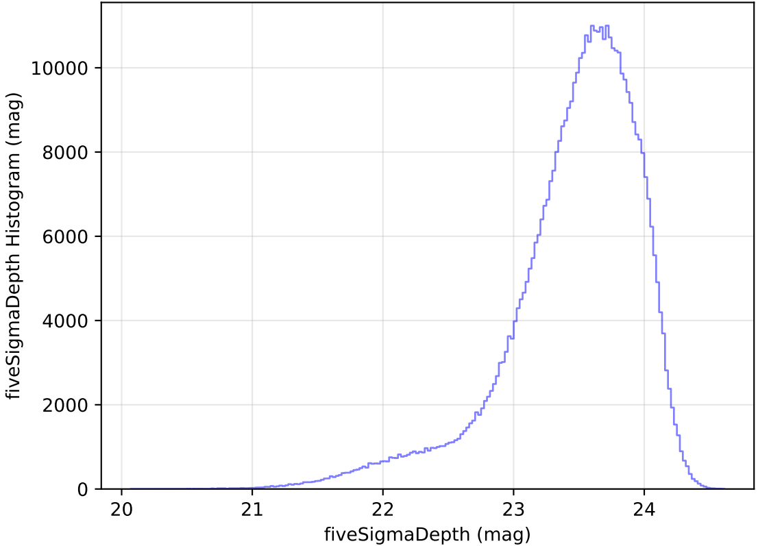
too_elab_r32_d2_ugrizy_v3.4_10yrs All sky i band: fiveSigmaDepth Histogram
