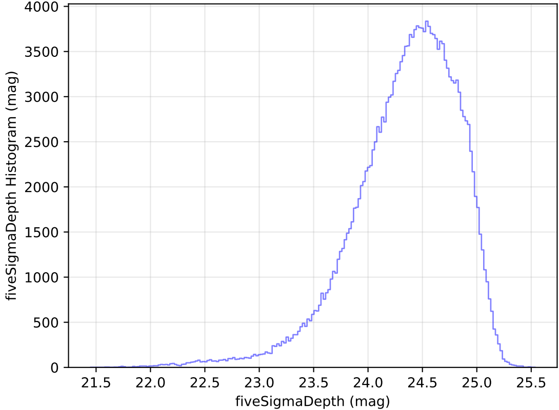
too_elab_r32_d2_ugrizy_v3.4_10yrs All sky g band: fiveSigmaDepth Histogram
