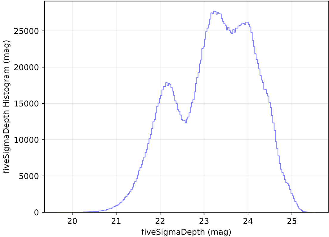
too_elab_r32_d2_ugrizy_v3.4_10yrs All sky all bands: fiveSigmaDepth Histogram
