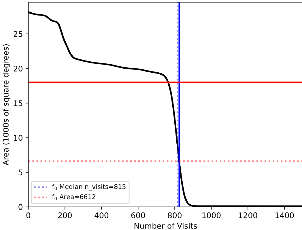
too_elab_r32_d2_ugrizy_v3.4_10yrs All sky: f0
