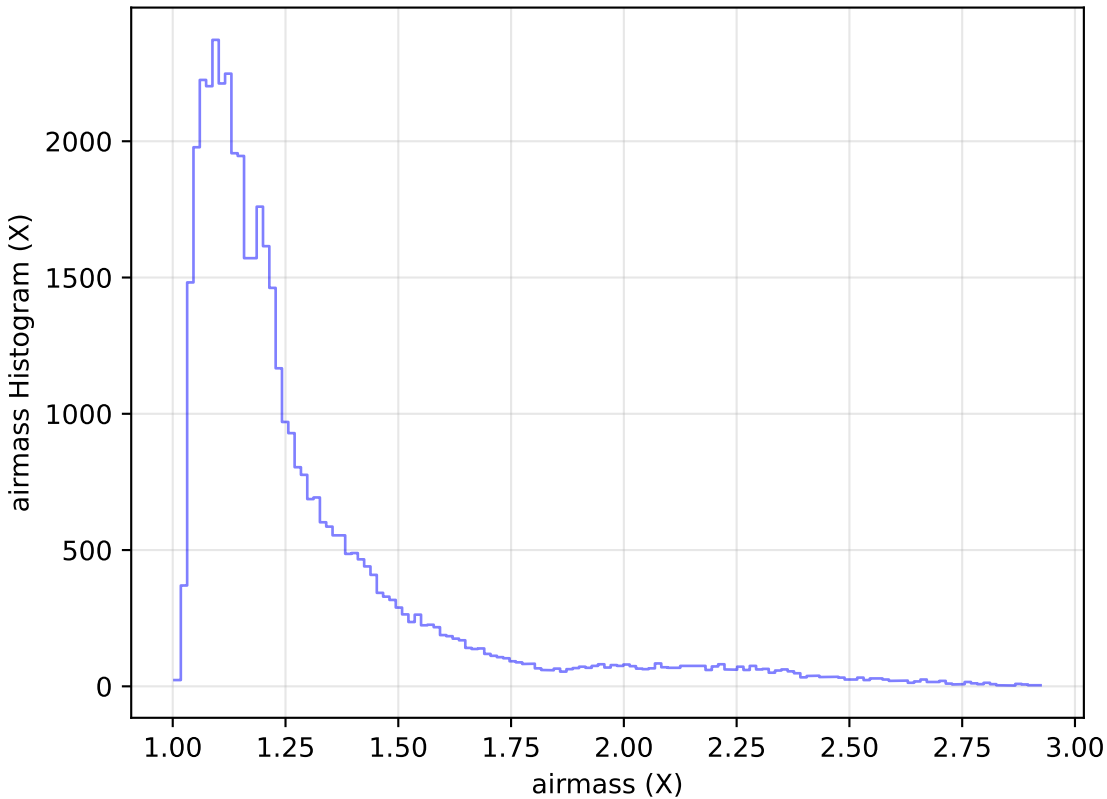
too_elab_r32_d2_ugrizy_v3.4_10yrs Yr 1 z band: airmass Histogram
