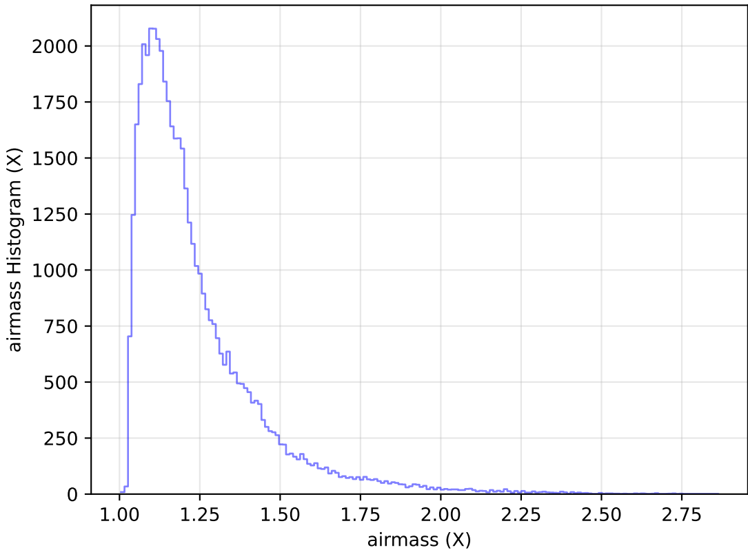
too_elab_r32_d2_ugrizy_v3.4_10yrs Yr 1 y band: airmass Histogram
