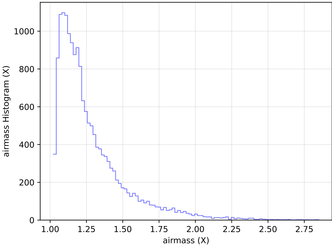
too_elab_r32_d2_ugrizy_v3.4_10yrs Yr 1 u band: airmass Histogram
