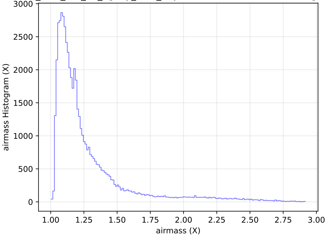
too_elab_r32_d2_ugrizy_v3.4_10yrs Yr 1 i band: airmass Histogram
