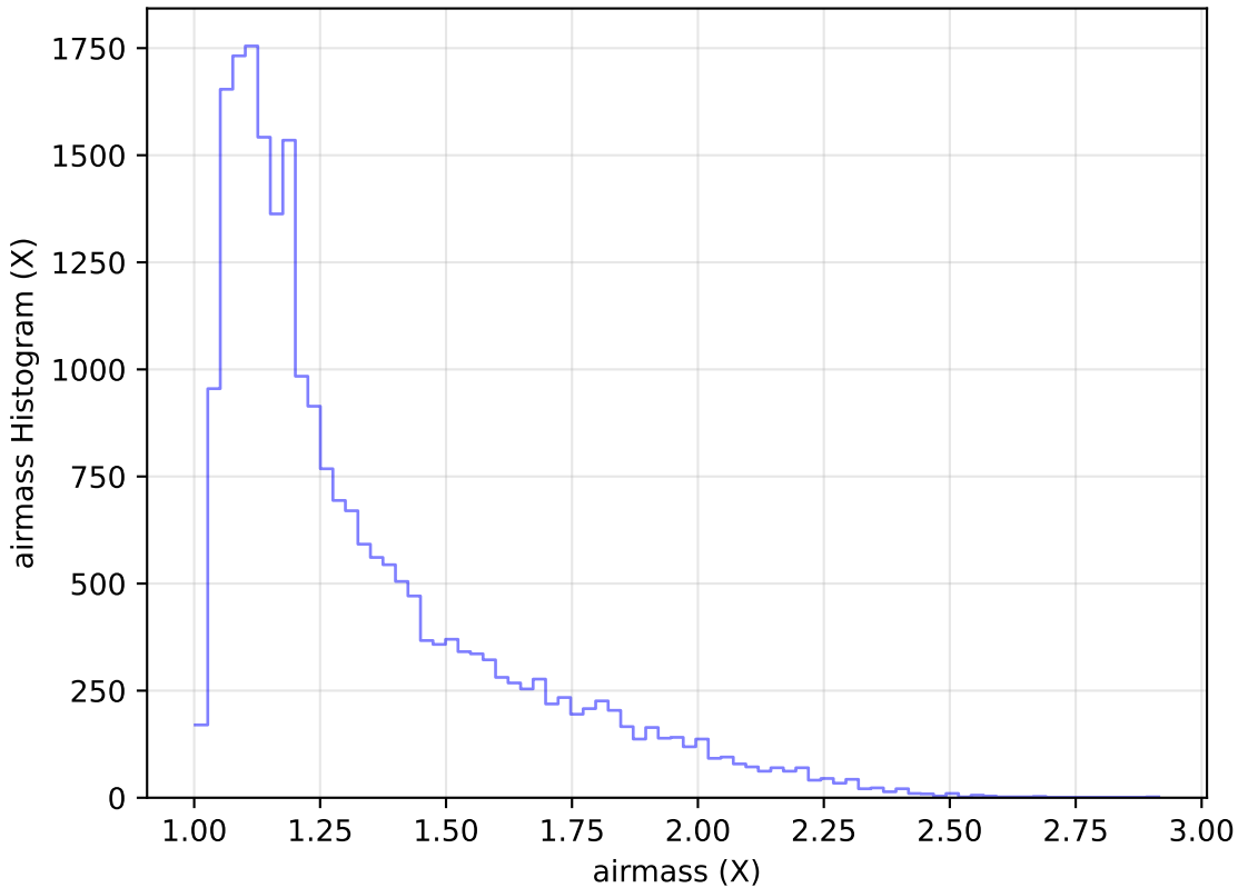
too_elab_r32_d2_ugrizy_v3.4_10yrs Yr 1 g band: airmass Histogram
