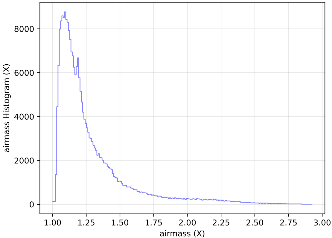
too_elab_r32_d2_ugrizy_v3.4_10yrs Yr 1 all bands: airmass Histogram
