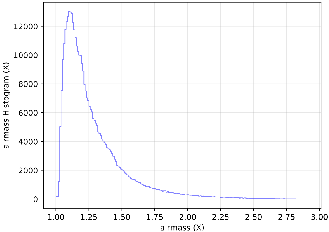
too_elab_r32_d2_ugrizy_v3.4_10yrs WFD y band: airmass Histogram
