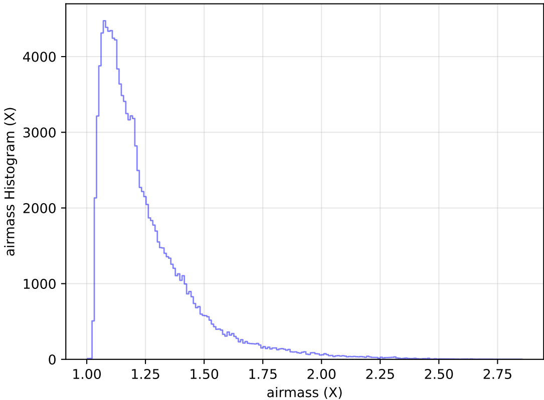
too_elab_r32_d2_ugrizy_v3.4_10yrs WFD u band: airmass Histogram
