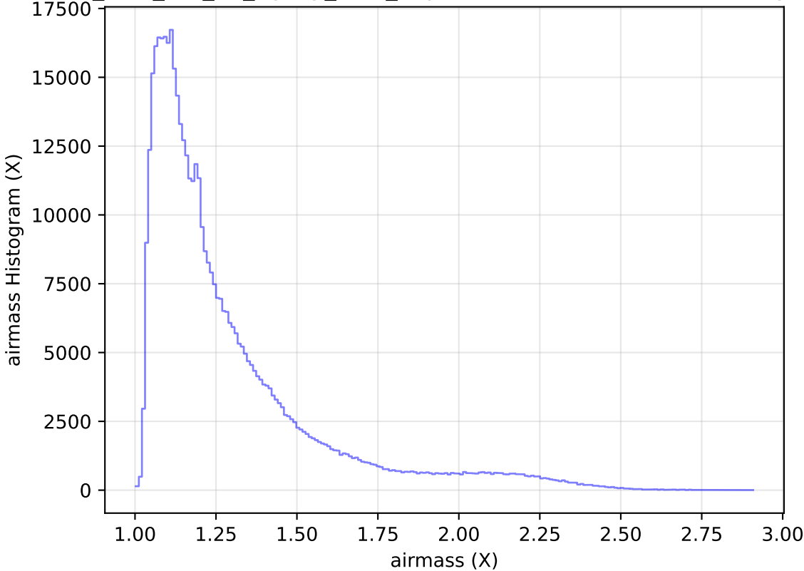
too_elab_r32_d2_ugrizy_v3.4_10yrs WFD r band: airmass Histogram
