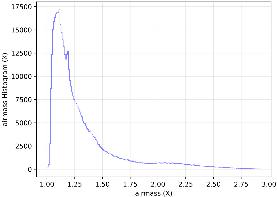
too_elab_r32_d2_ugrizy_v3.4_10yrs WFD i band: airmass Histogram
