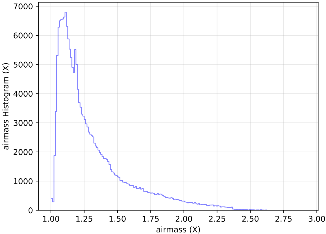
too_elab_r32_d2_ugrizy_v3.4_10yrs WFD g band: airmass Histogram
