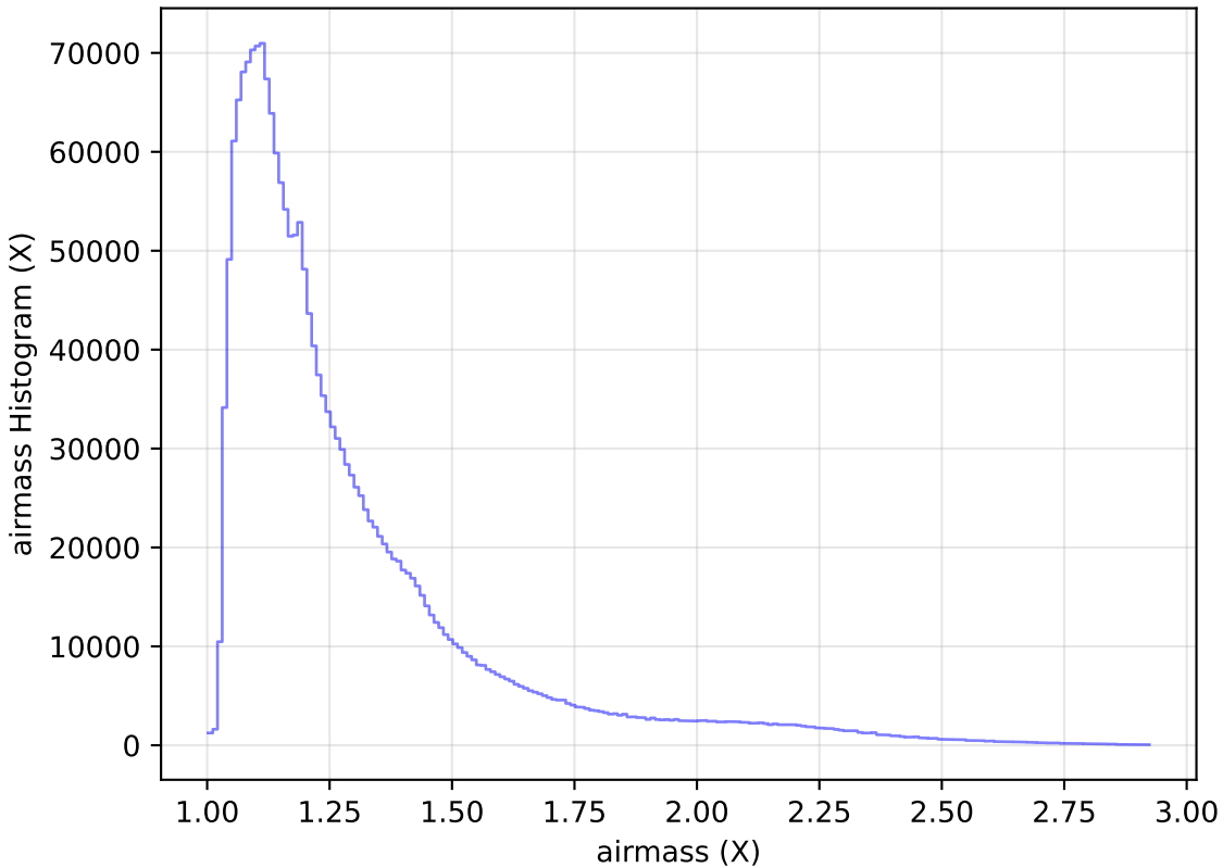
too_elab_r32_d2_ugrizy_v3.4_10yrs WFD all bands: airmass Histogram
