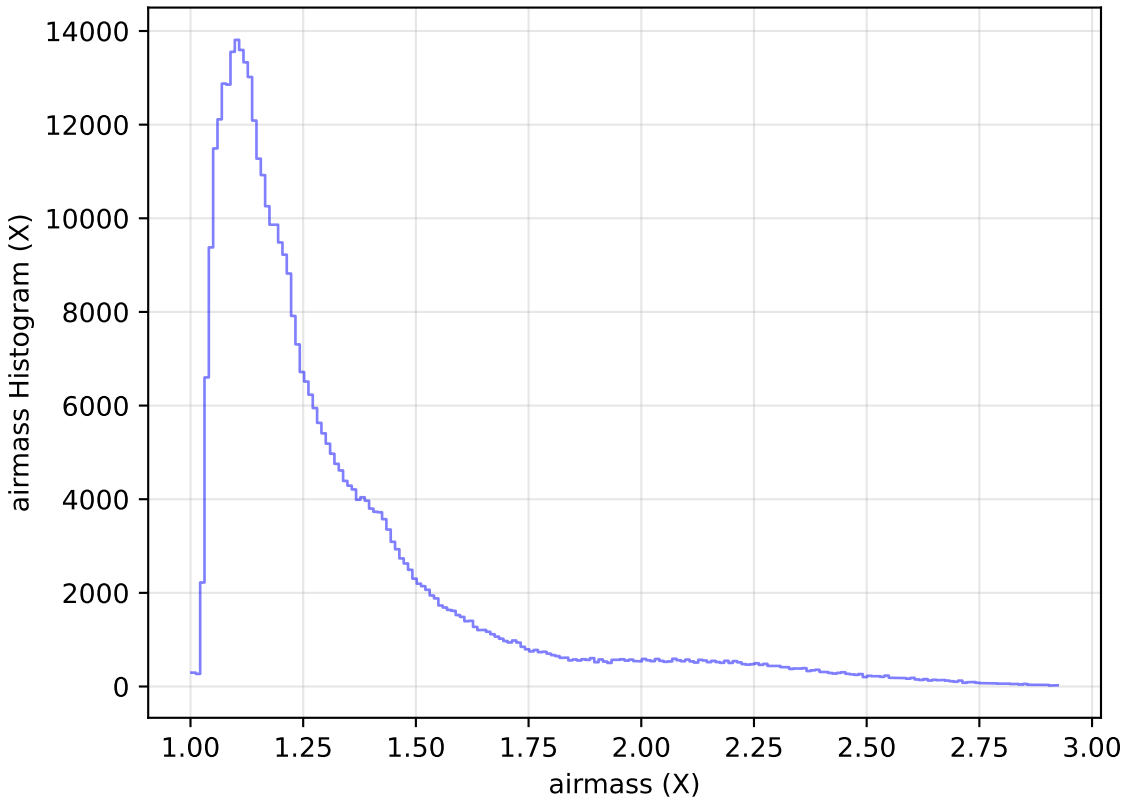
too_elab_r32_d2_ugrizy_v3.4_10yrs All sky z band: airmass Histogram
