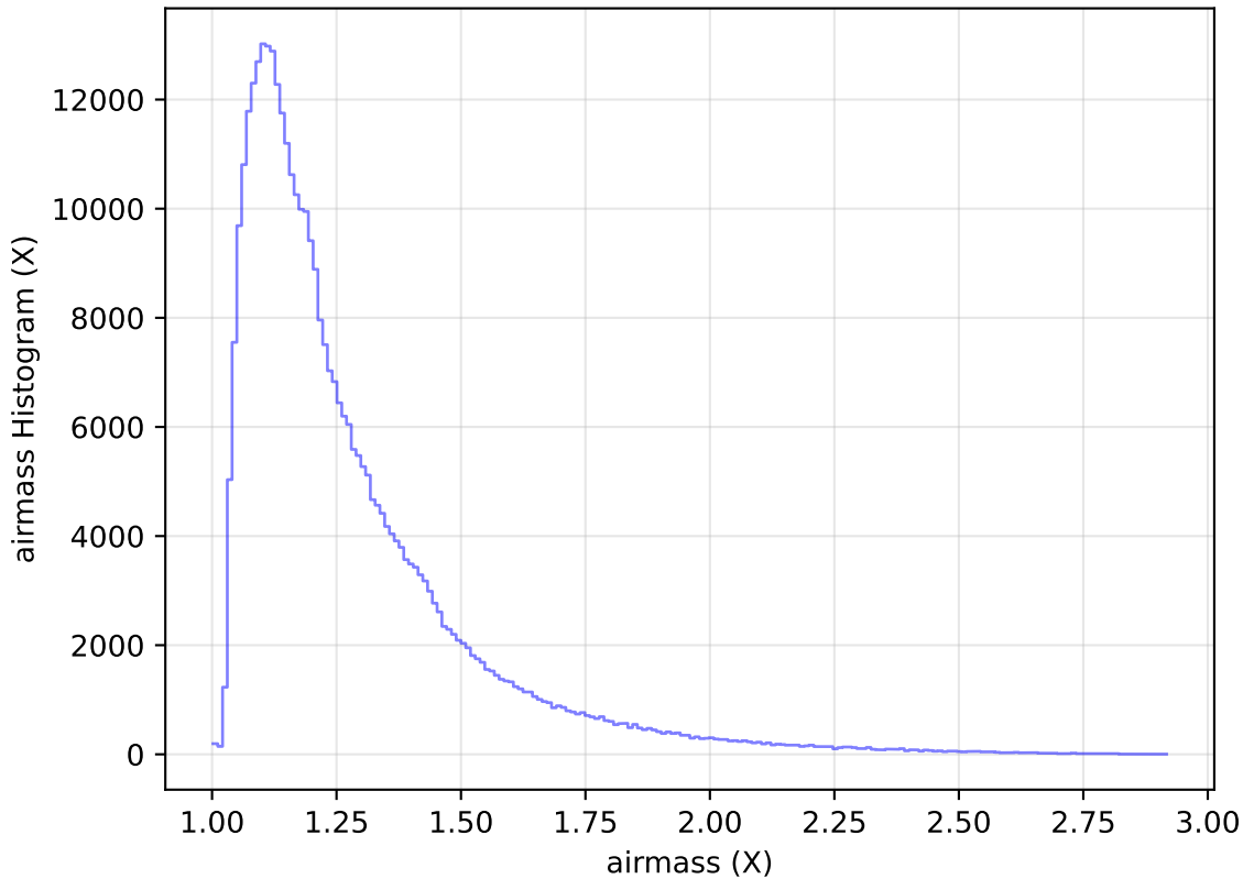
too_elab_r32_d2_ugrizy_v3.4_10yrs All sky y band: airmass Histogram
