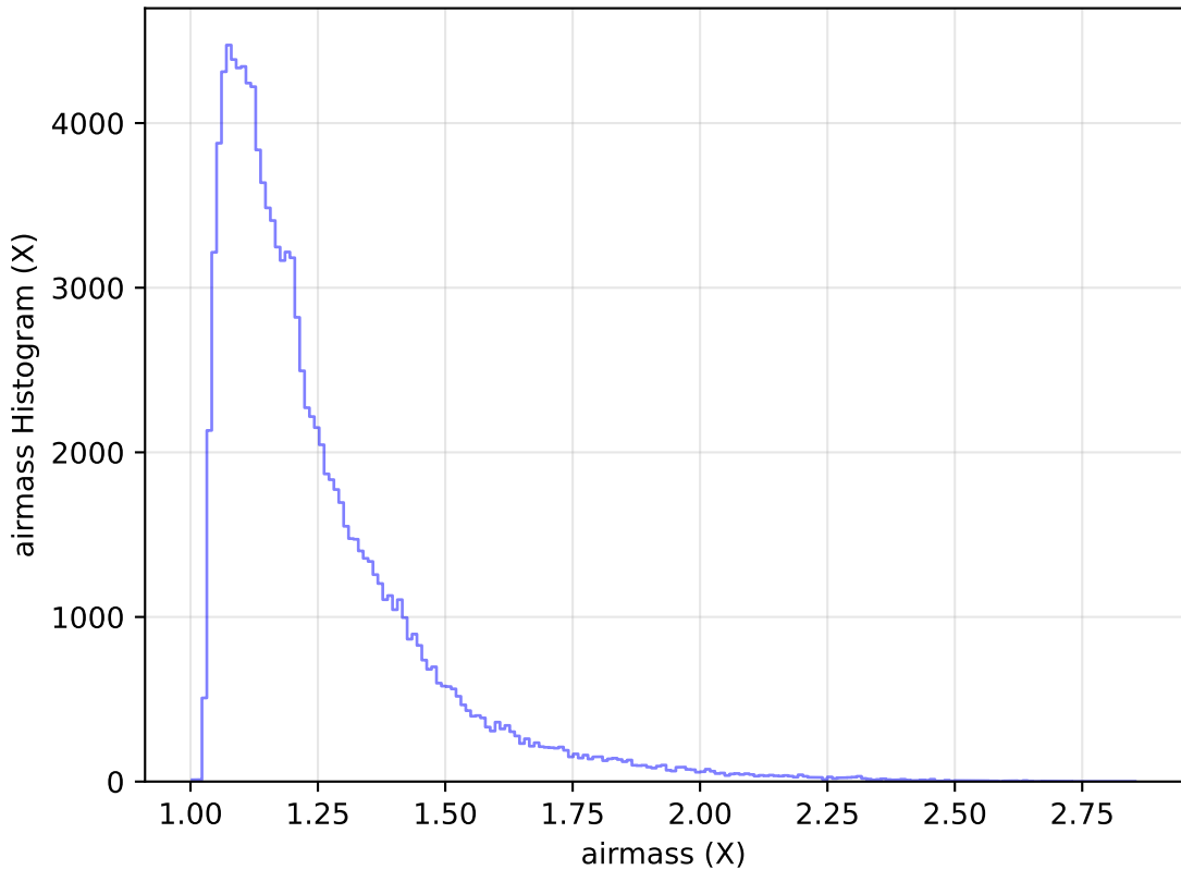
too_elab_r32_d2_ugrizy_v3.4_10yrs All sky u band: airmass Histogram
