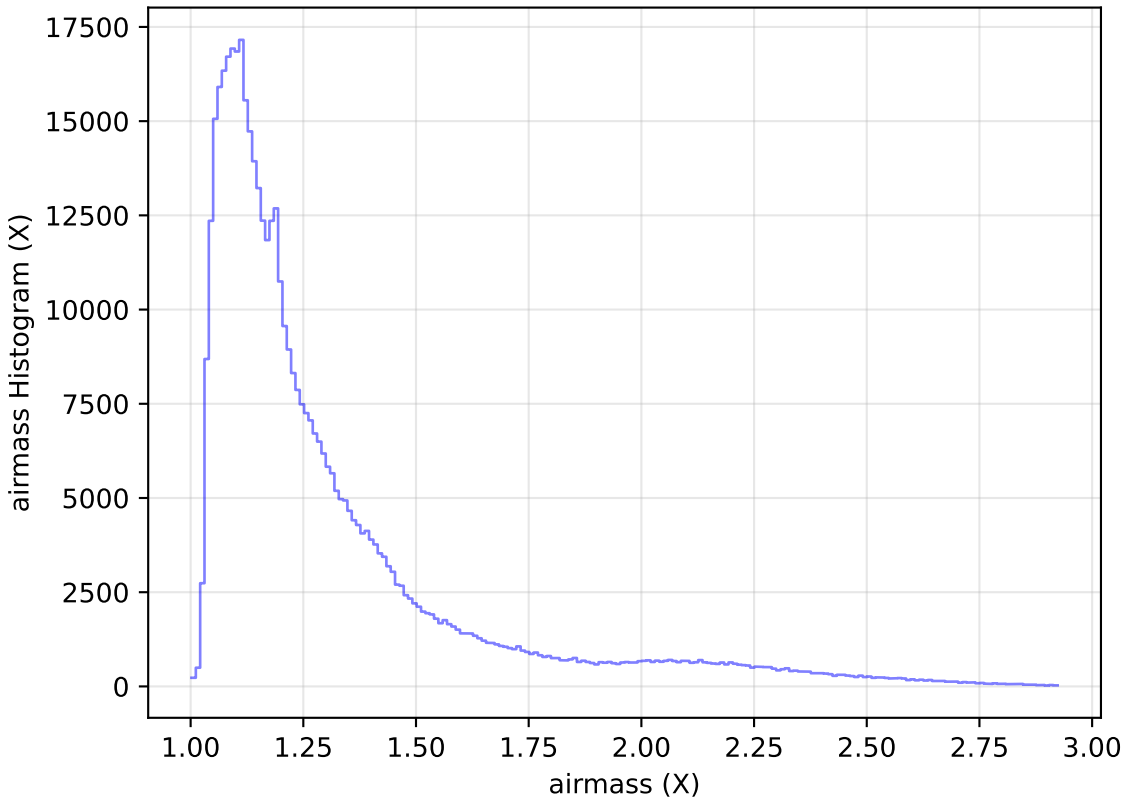
too_elab_r32_d2_ugrizy_v3.4_10yrs All sky i band: airmass Histogram
