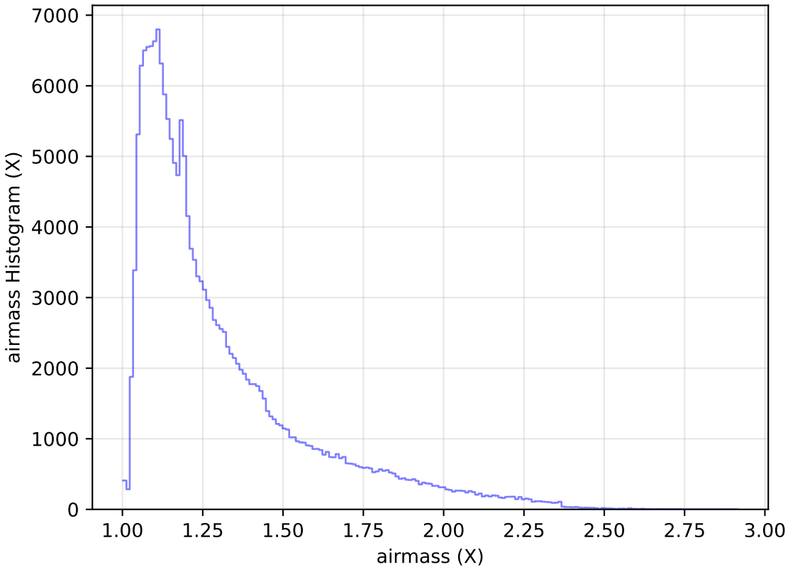
too_elab_r32_d2_ugrizy_v3.4_10yrs All sky g band: airmass Histogram
