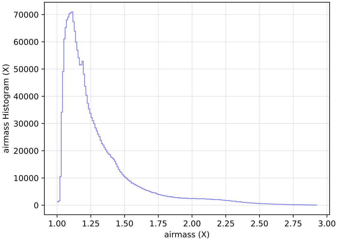
too_elab_r32_d2_ugrizy_v3.4_10yrs All sky all bands: airmass Histogram
