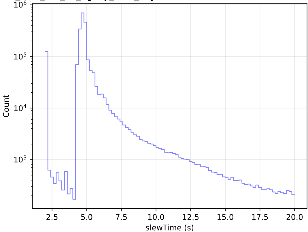
too_elab_r32_d2_ugrizy_v3.4_10yrs All visits: Zoom Slew Time Histogram
