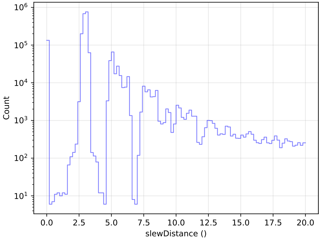
too_elab_r32_d2_ugrizy_v3.4_10yrs All visits: Zoom Slew Distance Histogram
