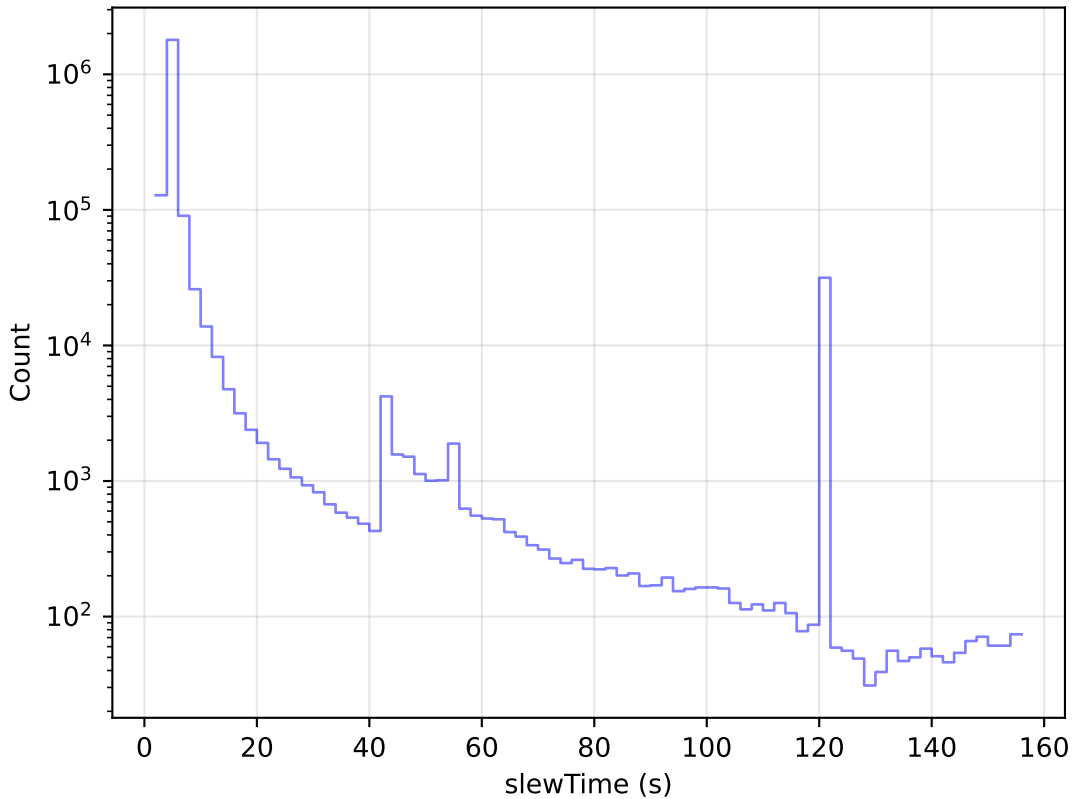
too_elab_r32_d2_ugrizy_v3.4_10yrs All visits: Slew Time Histogram
