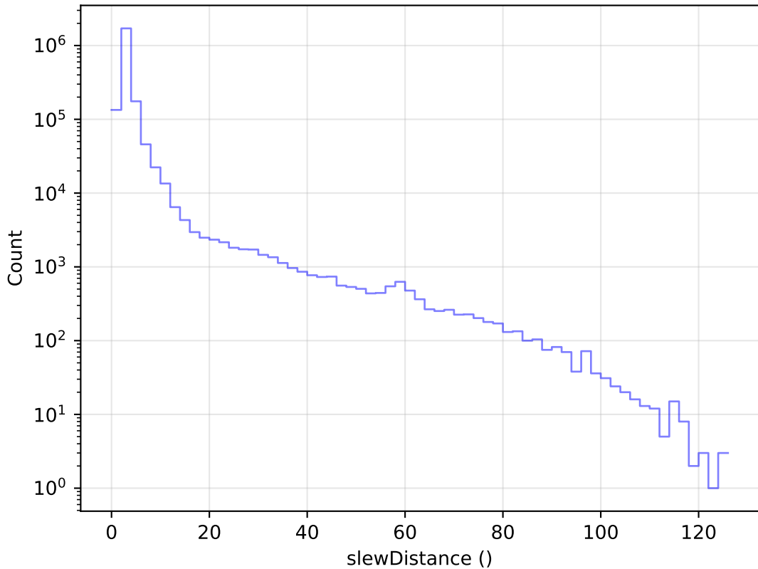
too_elab_r32_d2_ugrizy_v3.4_10yrs All visits: Slew Distance Histogram
