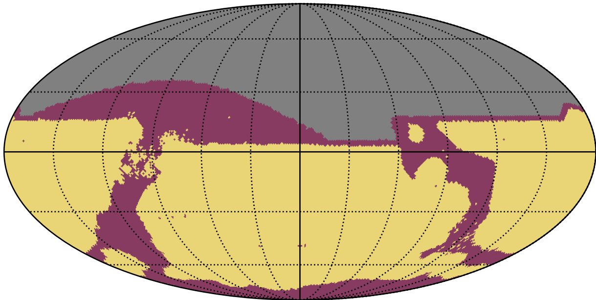
too_elab_r32_d2_ugrizy_v3.4_10yrs All sky: RapidRevisits
