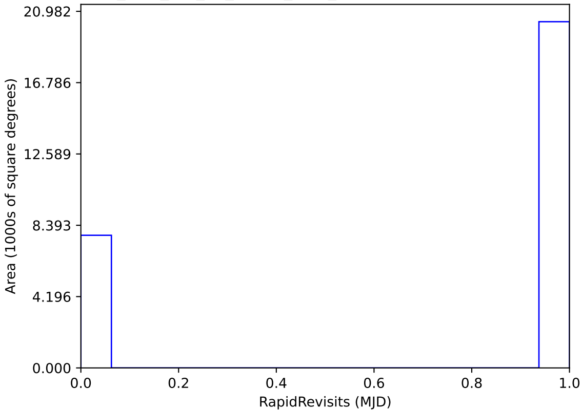
too_elab_r32_d2_ugrizy_v3.4_10yrs All sky: RapidRevisits
