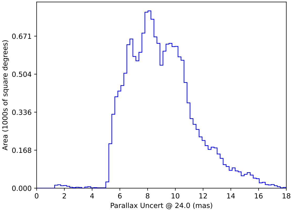
too_elab_r32_d2_ugrizy_v3.4_10yrs WFD: Parallax Uncert @ 24.0
